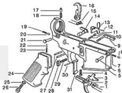
SGP15B FT parts Exploded View
